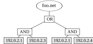
Fig. 3. The logical tree describing the MSQ of foo.net .
