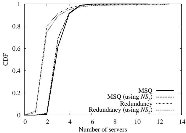
Fig. 4. The availability of a zone, in terms of MSQ and redundancy.
