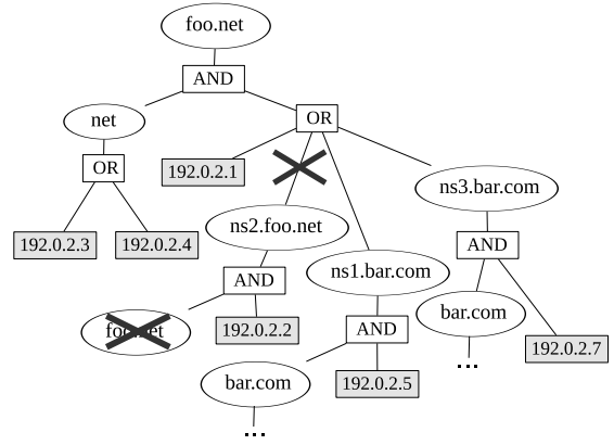
Fig. 2. A logical tree describing the availability of foo.net .
