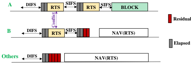
Fig. 2: An illustration of DC-PoET 1 mechanism.
