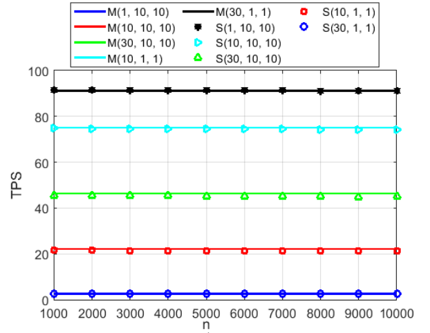
Fig. 5: Comparison of DC-PoET 1 with varying n ; simulations vs modeling. In this figure M and S denote “modeling” and “simulation”. The three parameters within braces are B (in MB), T (in minutes), and \sigma (in seconds).
